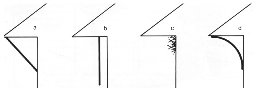
Figure 4. Four methods that may deter cliff swallow nesting: (a) netting attached from the outer edge of the eave down to the side of the building; (b) a curtain of netting; (c) metal projectors attached along the junction of the wall and eave; (d) a fiberglass panel mounted to form a smooth, concave surface.
